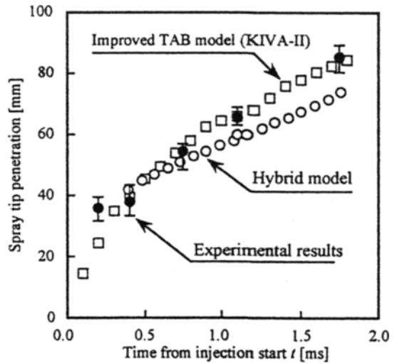
Fig. 17 Temporal change in spray tip penetration for computational and experimental results
