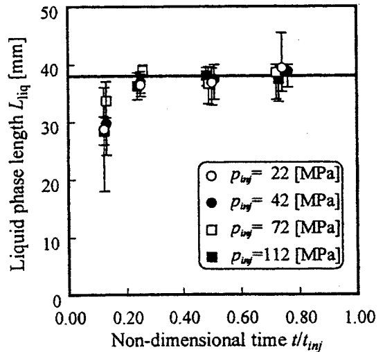
Fig. 10 Temporal change in liquid phase length
