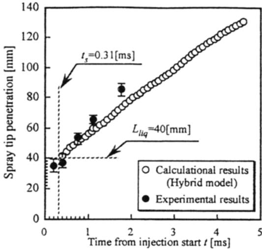
Fig. 14 Temporal change in spray tip penetration for calculation and experiment results
