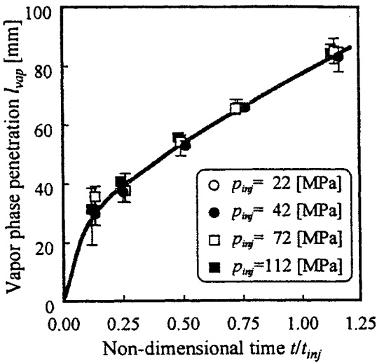
(a) Vapor phase penetration l_{vap}
