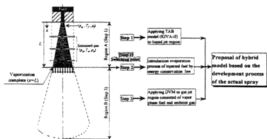
Fig. 1 Hypothesized spray structure with two-regions for simulation
