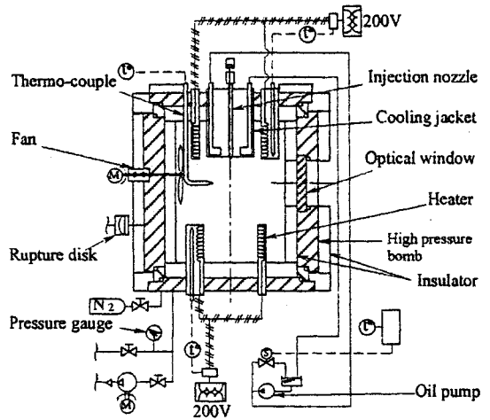
Fig. 3 Experimental apparatus
