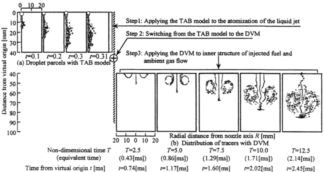
Fig. 13 Temporal change in droplet parcels with TAB model and distribution of tracers with DVM ( H=11 [mm], U_0=64.2 [m/s], \nu_g=1.99 \times 10^{-6} [m 2 /s], Re=3.55 \times 10^5 , T_{sv}=10.0 (1.71 [ms]))
