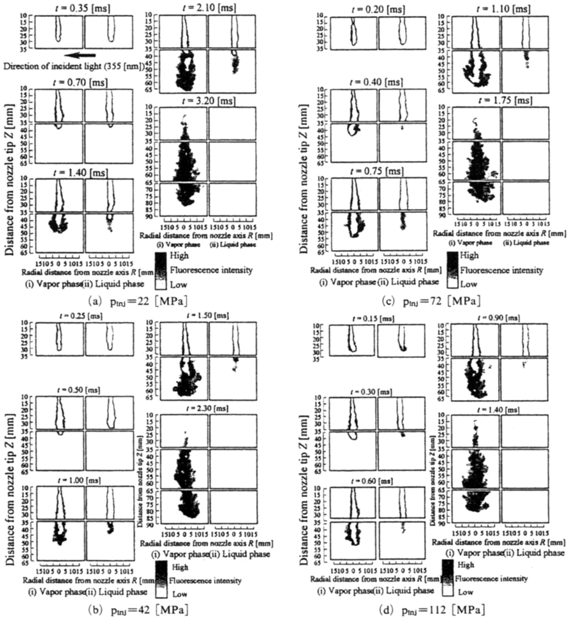
Fig. 8 Temporal change in free spray image with exciplex fluorescence method ( Q_{inj}=12.0 [mg], \rho_a=12.3 [kg/m 3 ], T_a=700 [K])
