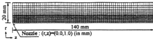
Fig. 7 Computational mesh
