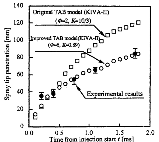
Fig. 6 Temporal change in spray tip penetration for calculational and experimental results
