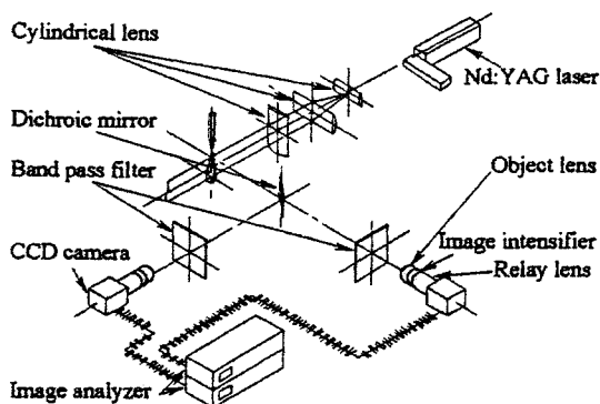
Fig. 4 Schematic diagram of laser sheet optical system and photography system
