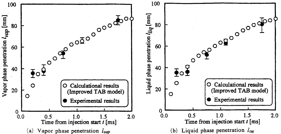
Fig. 12 Temporal change in penetration of vapor and liquid phase ( p_{nv}=72 [Mpa], \rho_a=12.3 [kg/m 3 ])
