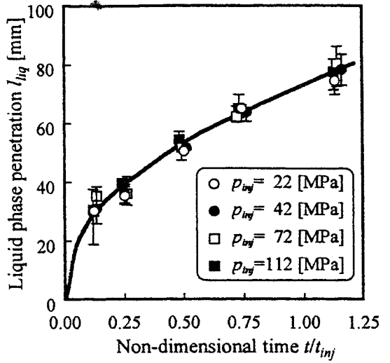
(b) Liquid phase penetration l_{liq}
