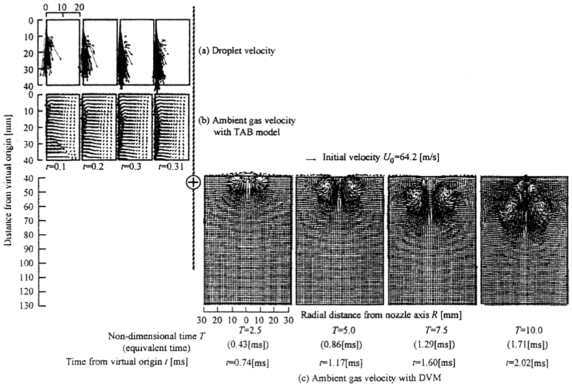
Fig. 15 Temporal change in droplet proplet velocity and ambient gas velocity TAB model and ambient gas velocity with DVM
