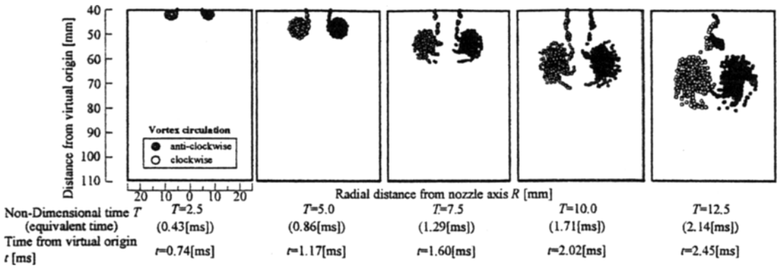
Fig. 16 Temporal change in distribution of vortices
